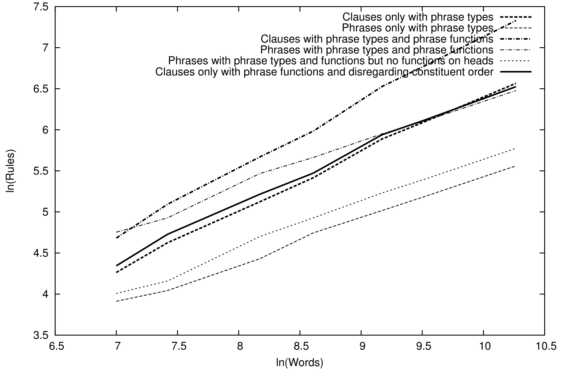
Plot of \ln of rules against \ln of words
