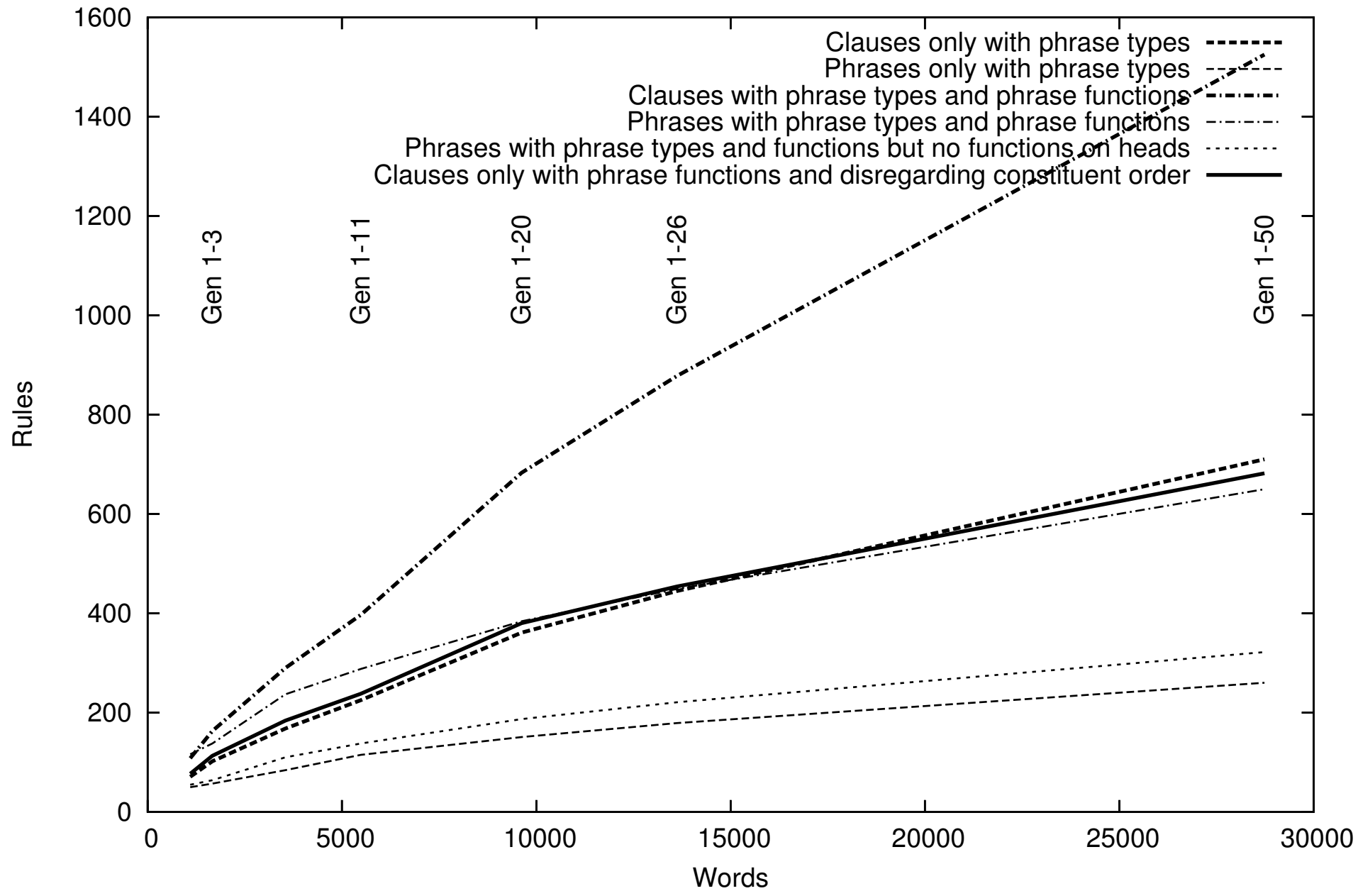
Plot of rules against words
